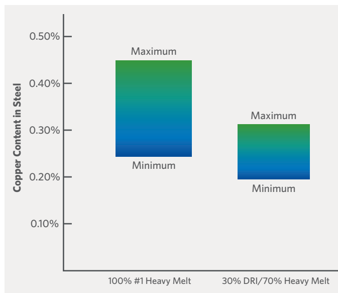
FIGURE 3. Influence of DRI on copper variability
