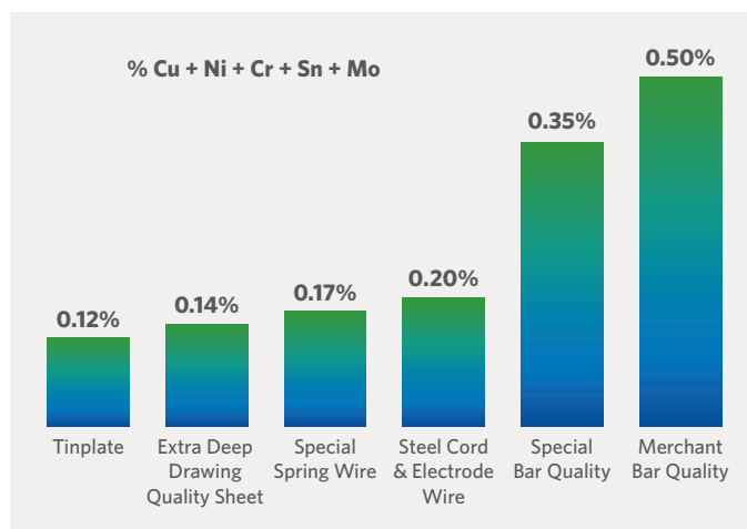
FIGURE 2. Typical residual limits in carbon steel products
