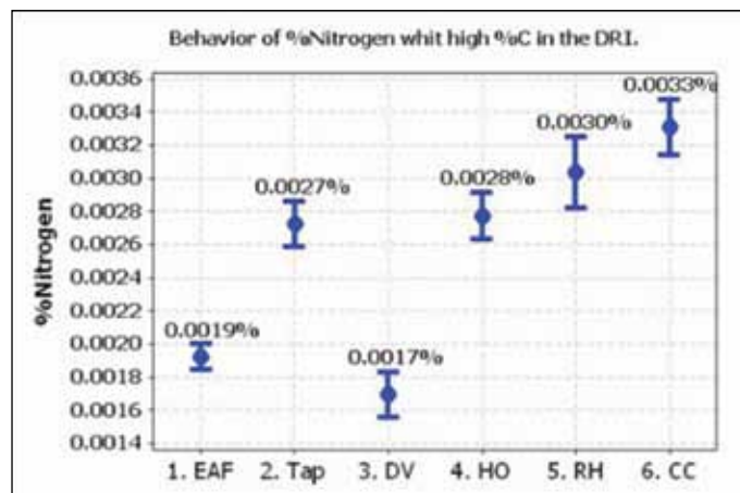
FIGURE 8 Nitrogen behavior in each process stage (100% DRI)
