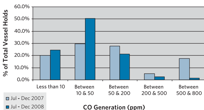
FIGURE 1 Graph of Carbon Monoxide generation by vessel hold for July - December 2007 & 2008
